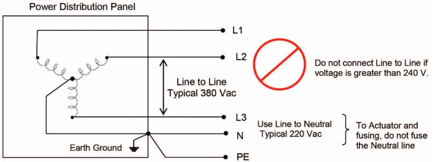
Grounded WYE Power Connection, 220/380Y 3Φ
