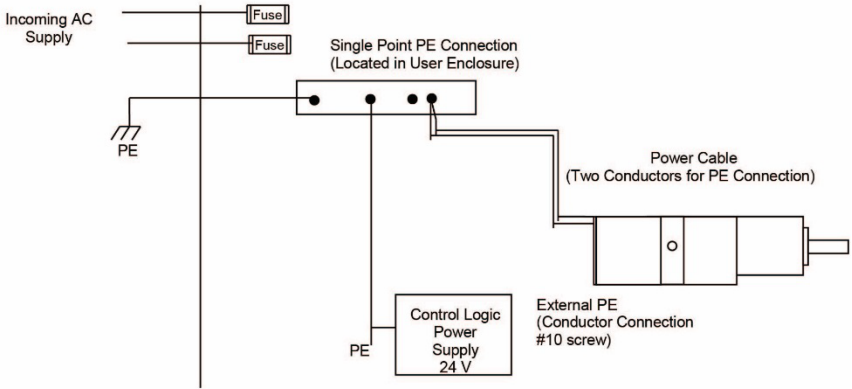
Grounding Schematic
