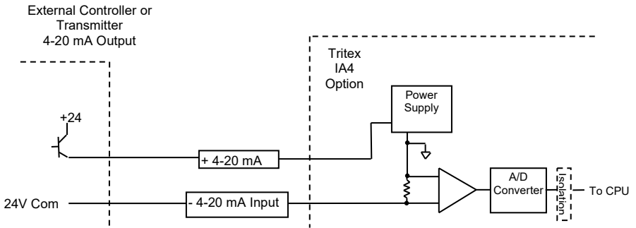
Connection to High Side Controller
